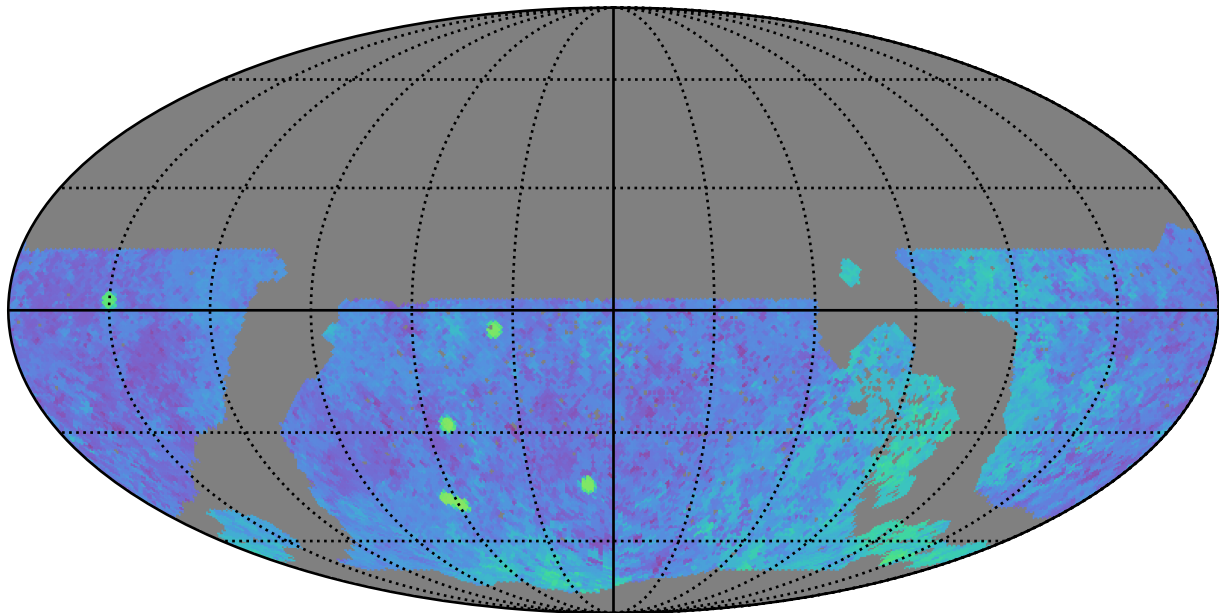
noroll_mjdp120_v3.4_10yrs WFD g band: Median Season Length
