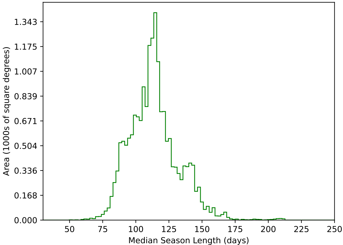
noroll_mjdp120_v3.4_10yrs WFD g band: Median Season Length
