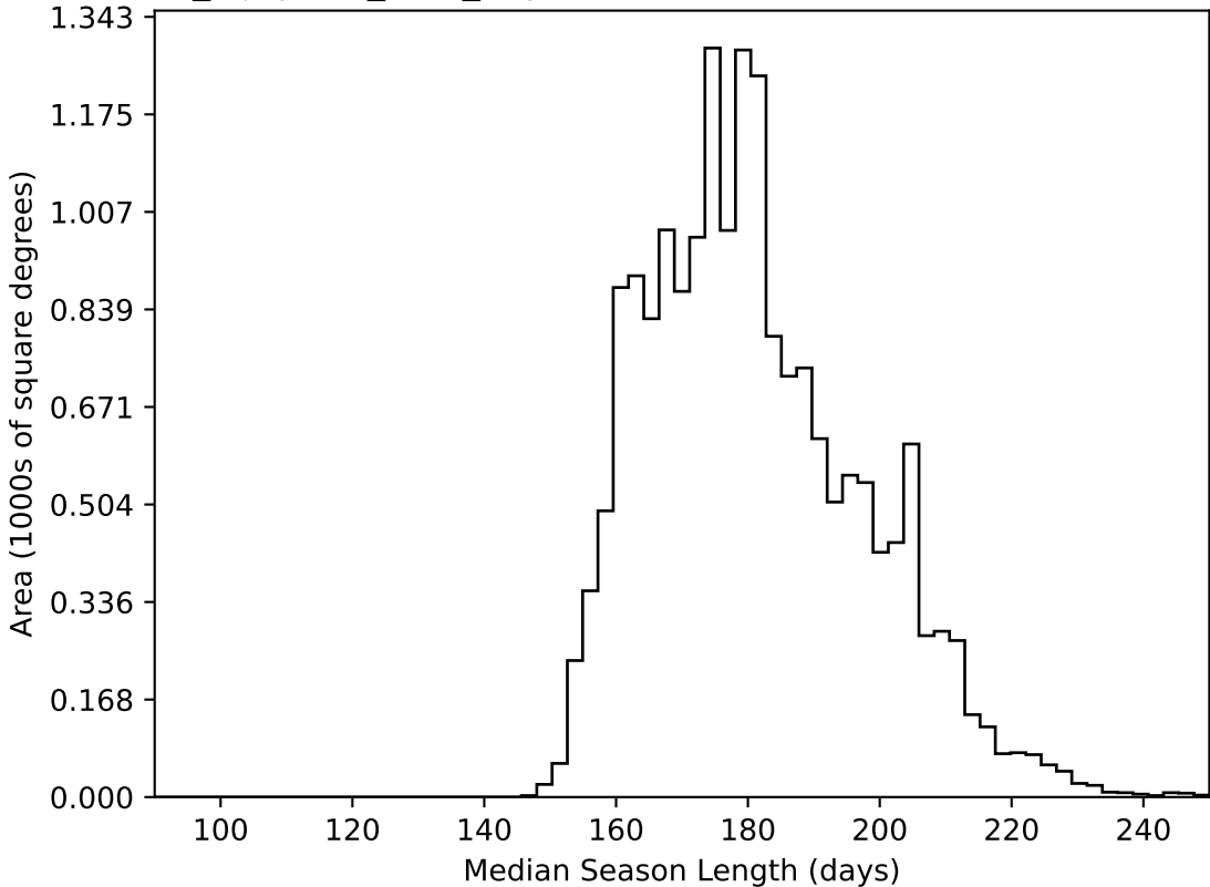
noroll_mjdp120_v3.4_10yrs WFD all bands: Median Season Length
