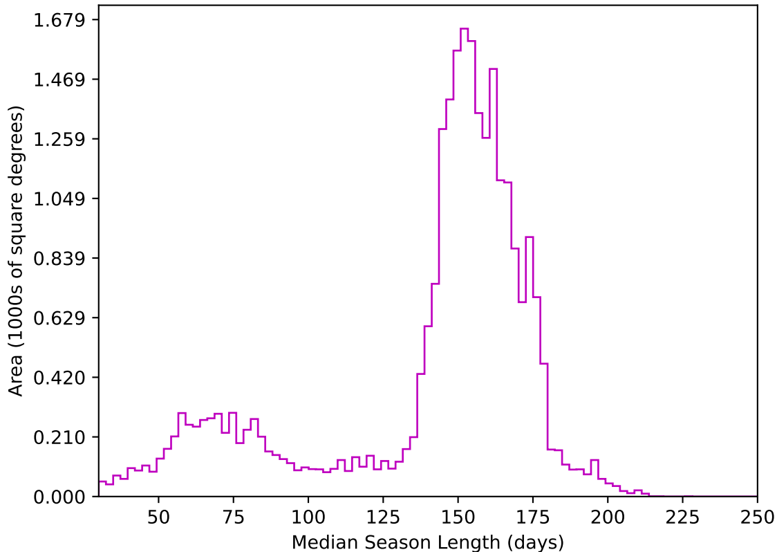
noroll_mjdp120_v3.4_10yrs All sky z band: Median Season Length
