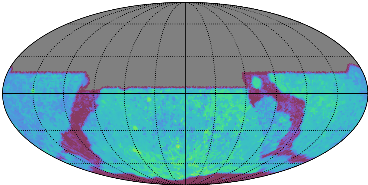
noroll_mjdp120_v3.4_10yrs All sky y band: Median Season Length
