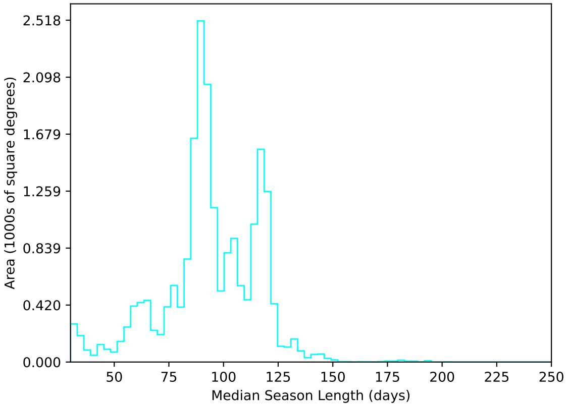
noroll_mjdp120_v3.4_10yrs All sky u band: Median Season Length
