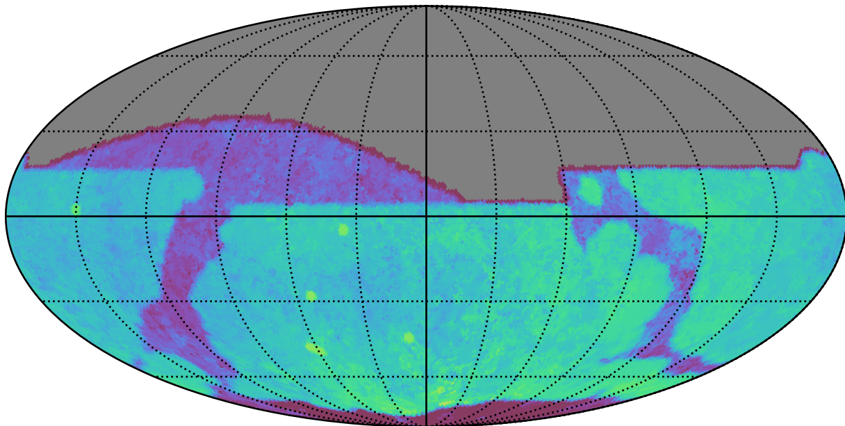
noroll_mjdp120_v3.4_10yrs All sky r band: Median Season Length
