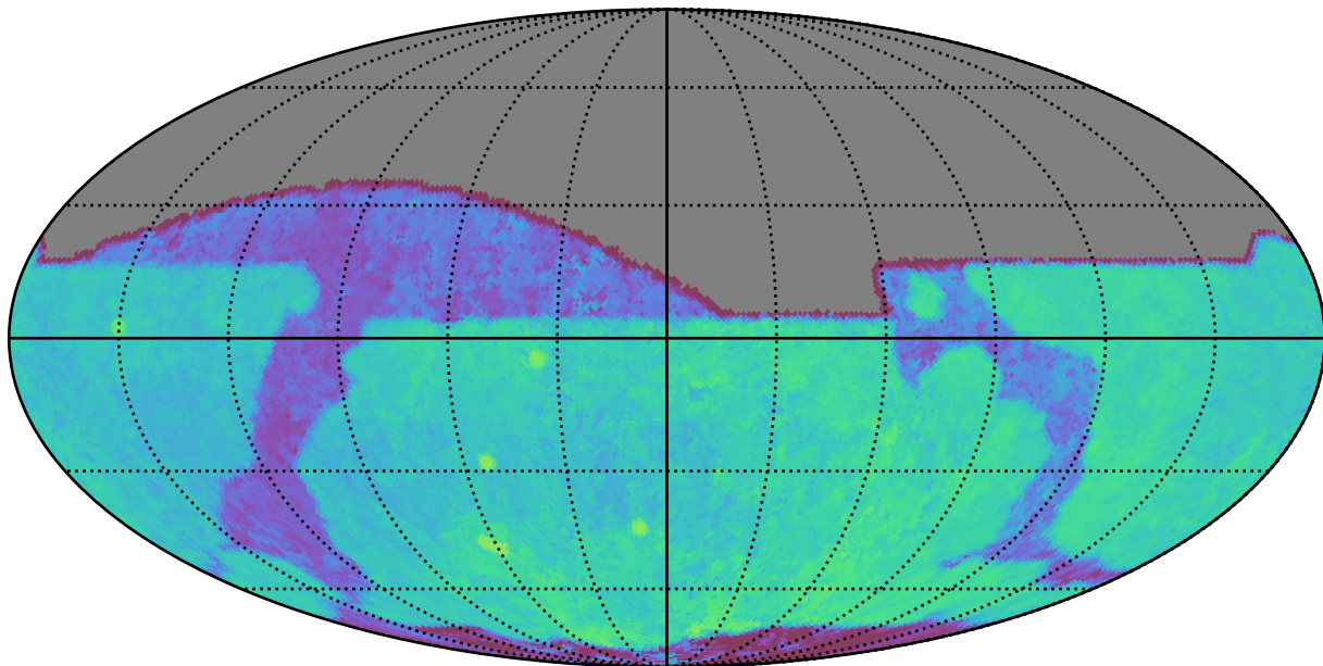
noroll_mjdp120_v3.4_10yrs All sky i band: Median Season Length
