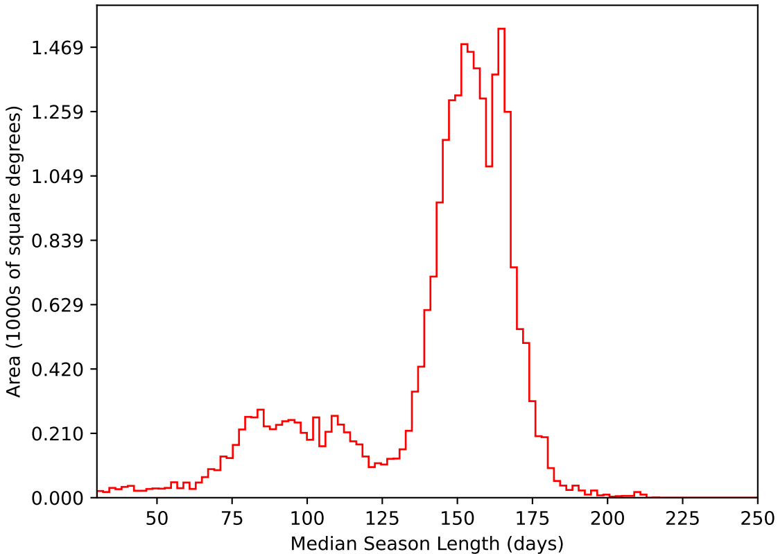
noroll_mjdp120_v3.4_10yrs All sky i band: Median Season Length
