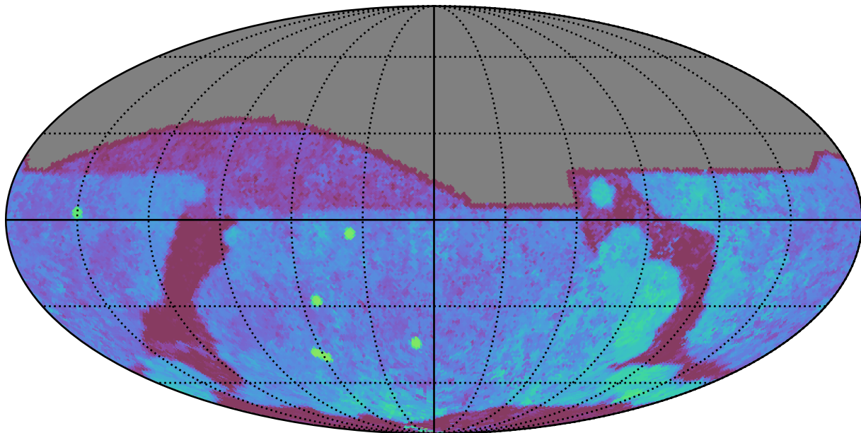
noroll_mjdp120_v3.4_10yrs All sky g band: Median Season Length
