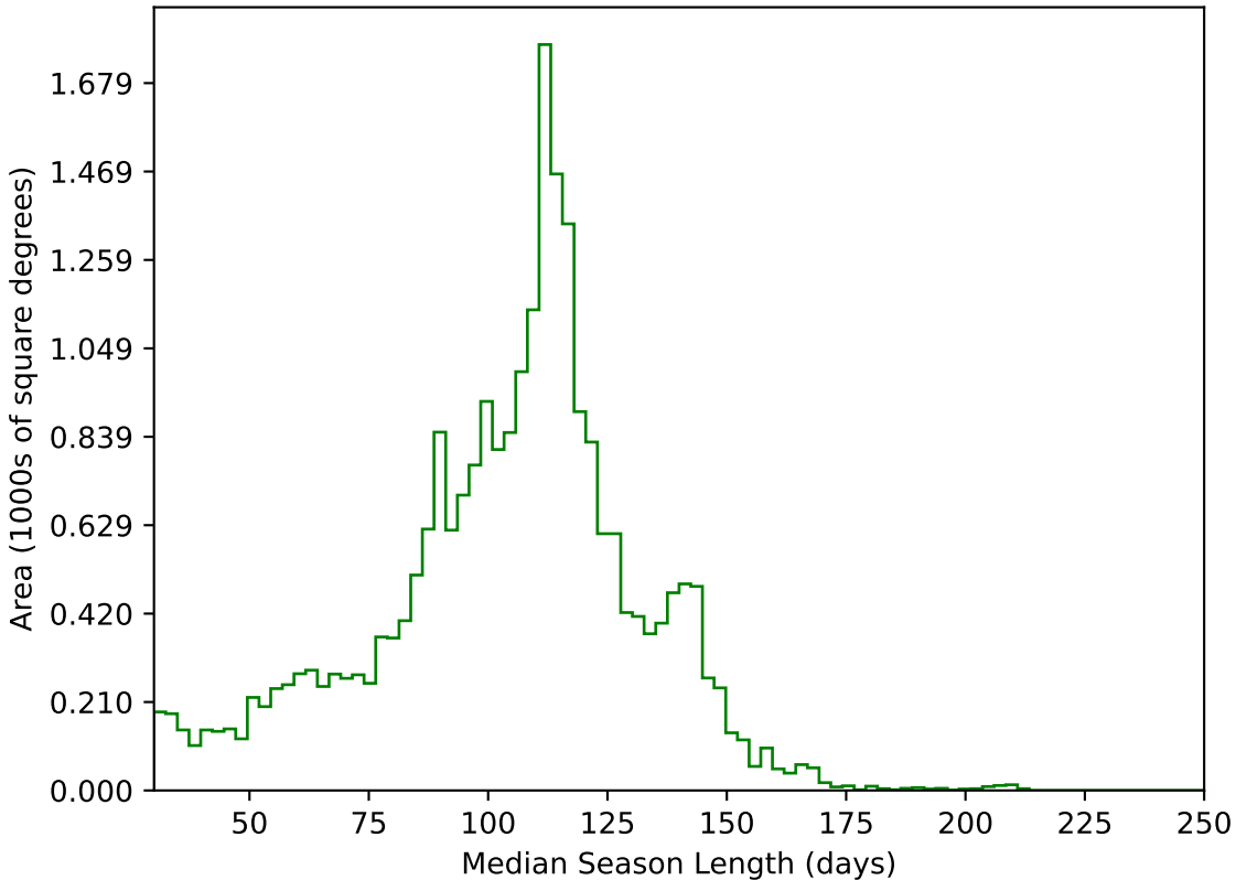
noroll_mjdp120_v3.4_10yrs All sky g band: Median Season Length
