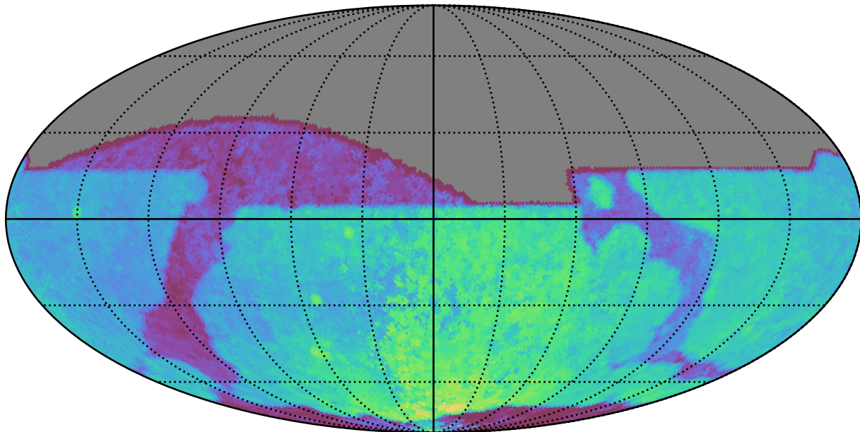
noroll_mjdp120_v3.4_10yrs All sky all bands: Median Season Length
