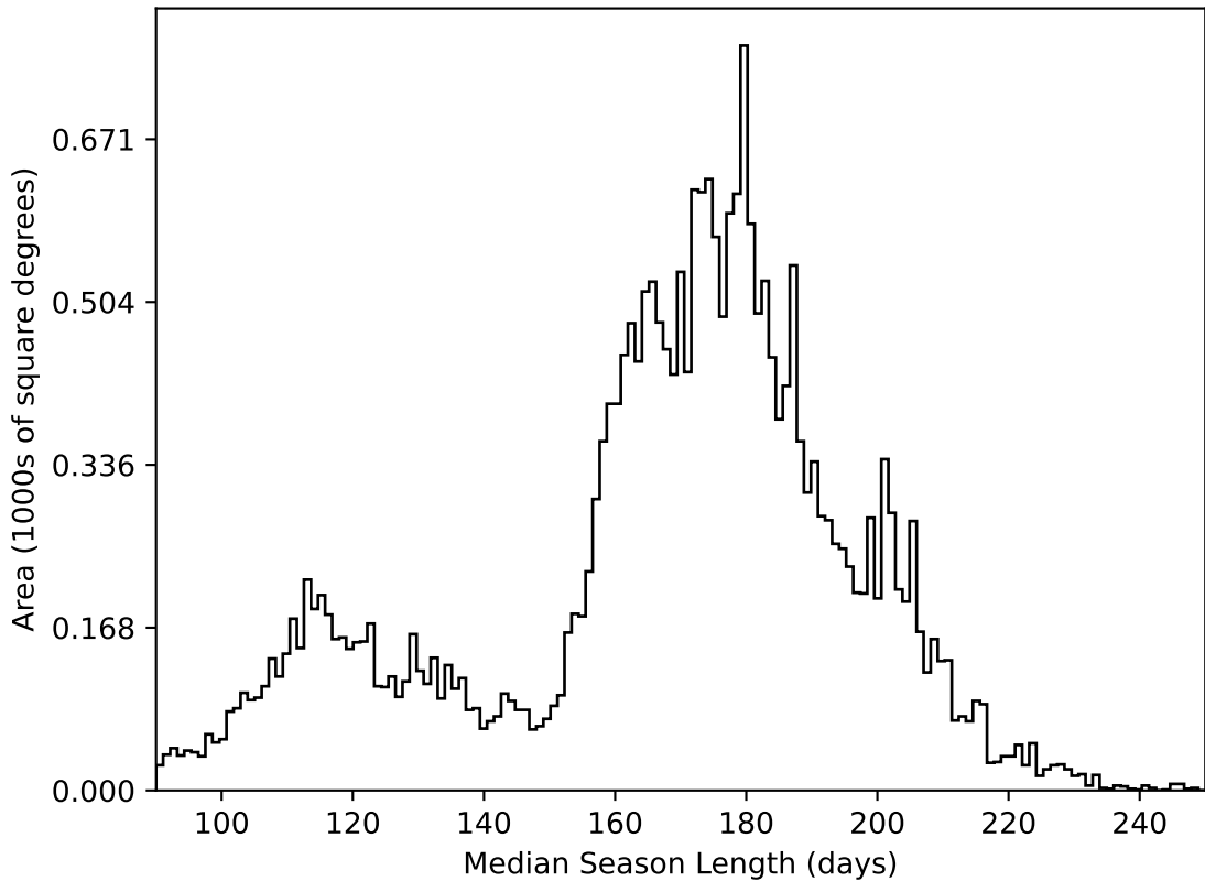
noroll_mjdp120_v3.4_10yrs All sky all bands: Median Season Length
