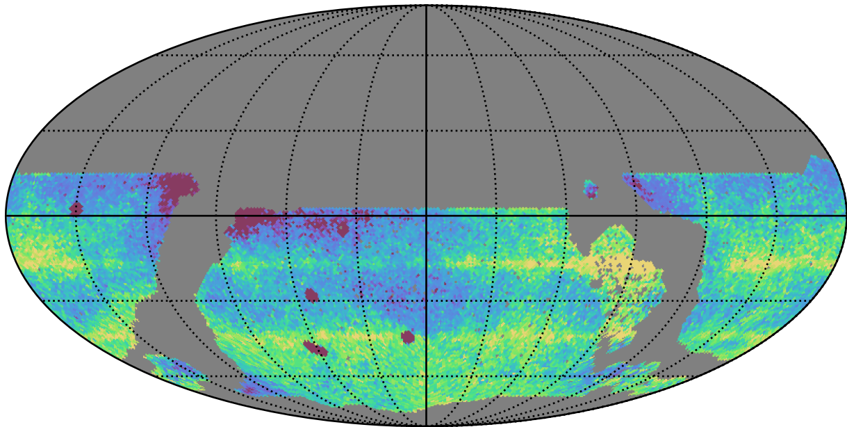
noroll_mjdp120_v3.4_10yrs WFD: Median Intra-Night Gap
