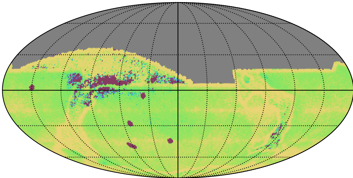
noroll_mjdp120_v3.4_10yrs All sky: Median Intra-Night Gap
