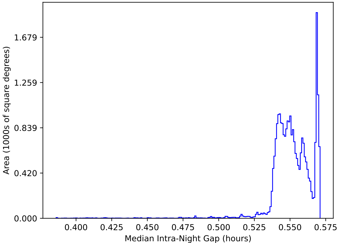
noroll_mjdp120_v3.4_10yrs All sky: Median Intra-Night Gap
