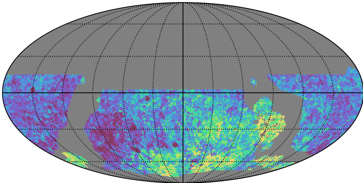
noroll_mjdp120_v3.4_10yrs WFD z band: Median Inter-Night Gap
