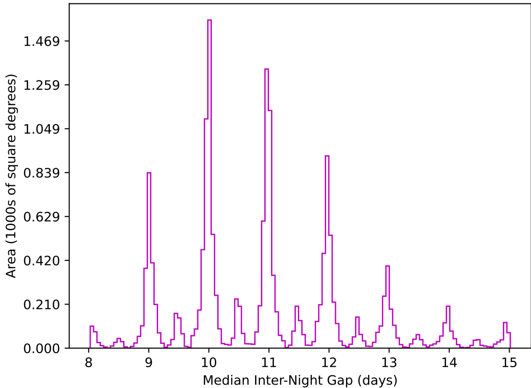
noroll_mjdp120_v3.4_10yrs WFD z band: Median Inter-Night Gap
