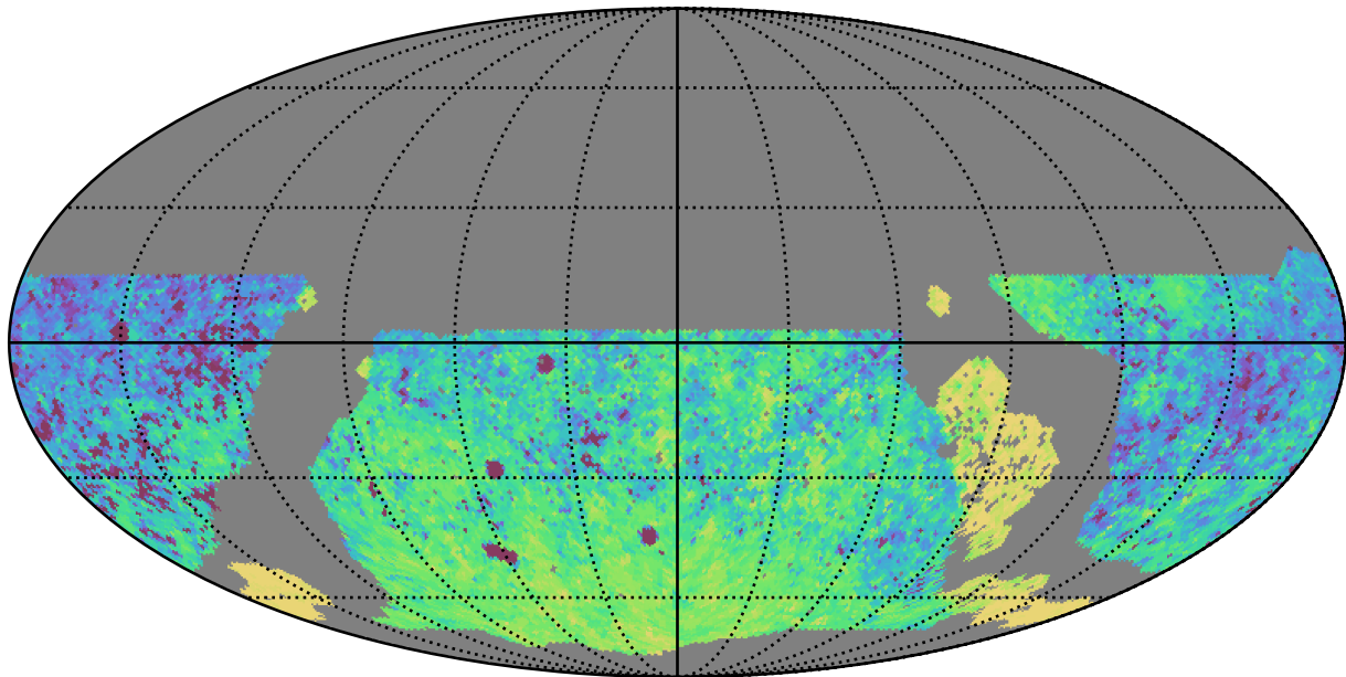
noroll_mjdp120_v3.4_10yrs WFD y band: Median Inter-Night Gap
