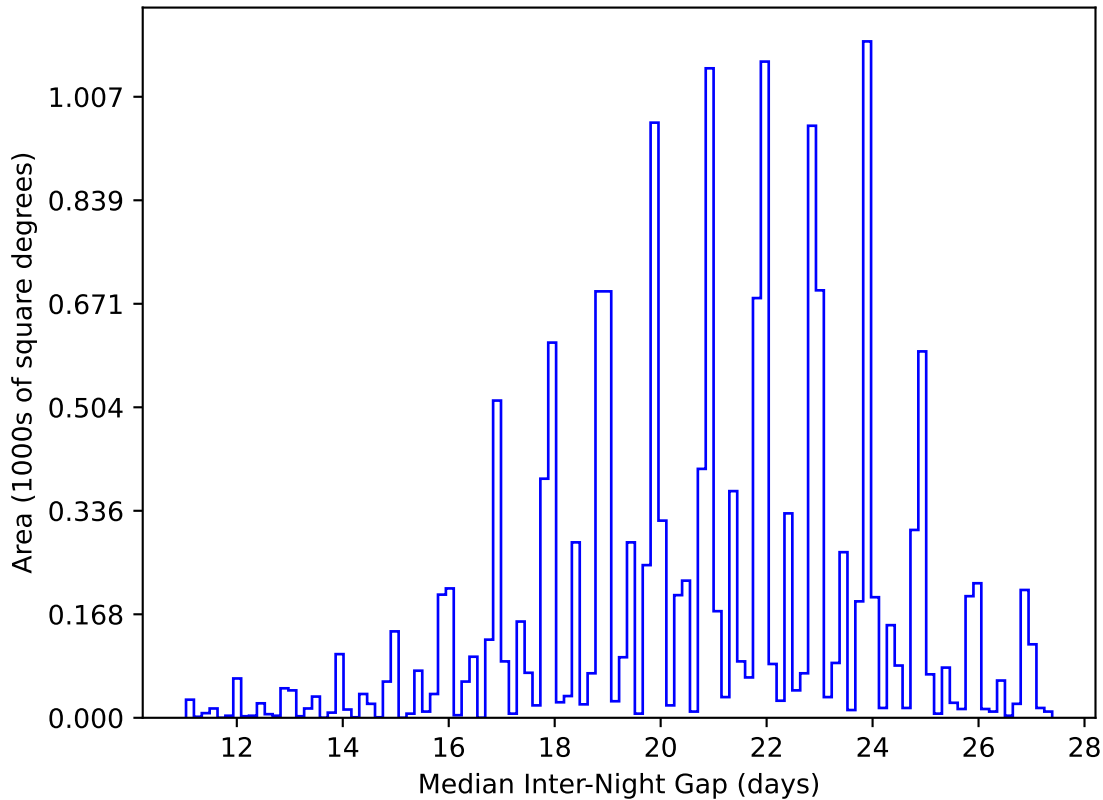
noroll_mjdp120_v3.4_10yrs WFD y band: Median Inter-Night Gap
