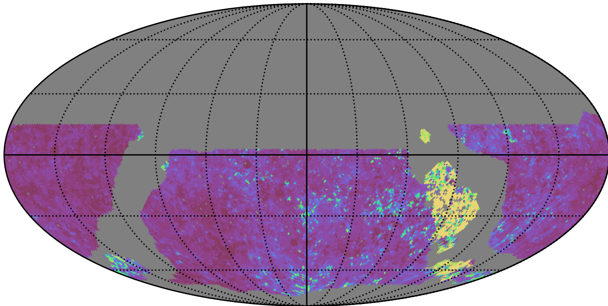
noroll_mjdp120_v3.4_10yrs WFD u band: Median Inter-Night Gap
