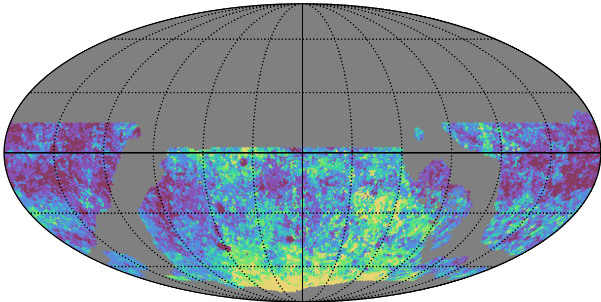
noroll_mjdp120_v3.4_10yrs WFD r band: Median Inter-Night Gap
