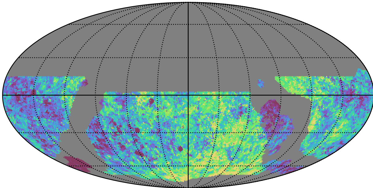
noroll_mjdp120_v3.4_10yrs WFD g band: Median Inter-Night Gap
