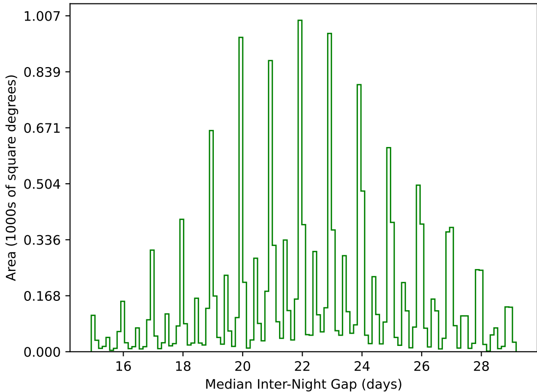
noroll_mjdp120_v3.4_10yrs WFD g band: Median Inter-Night Gap
