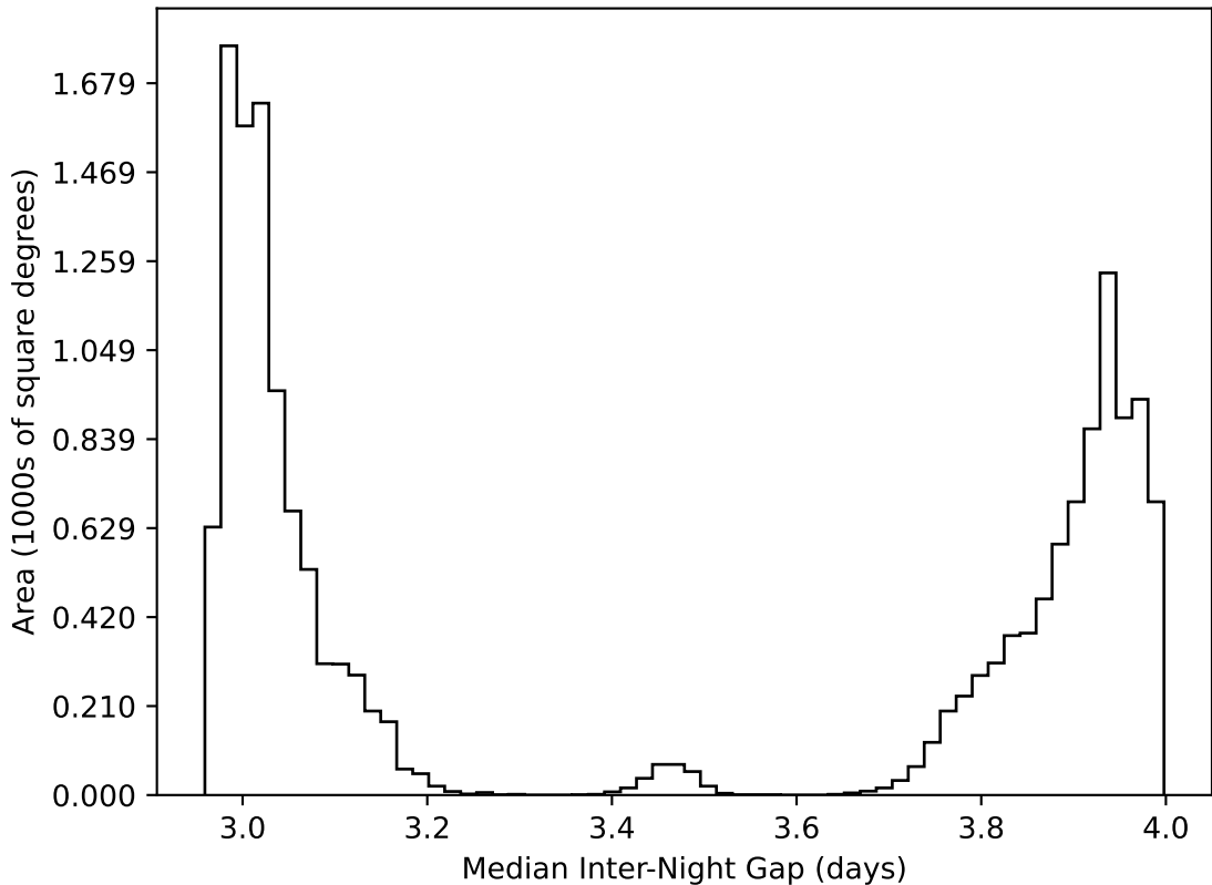
noroll_mjdp120_v3.4_10yrs WFD all bands: Median Inter-Night Gap
