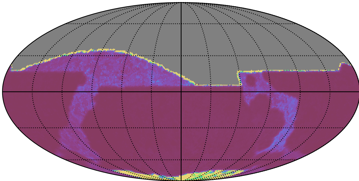
noroll_mjdp120_v3.4_10yrs All sky z band: Median Inter-Night Gap
