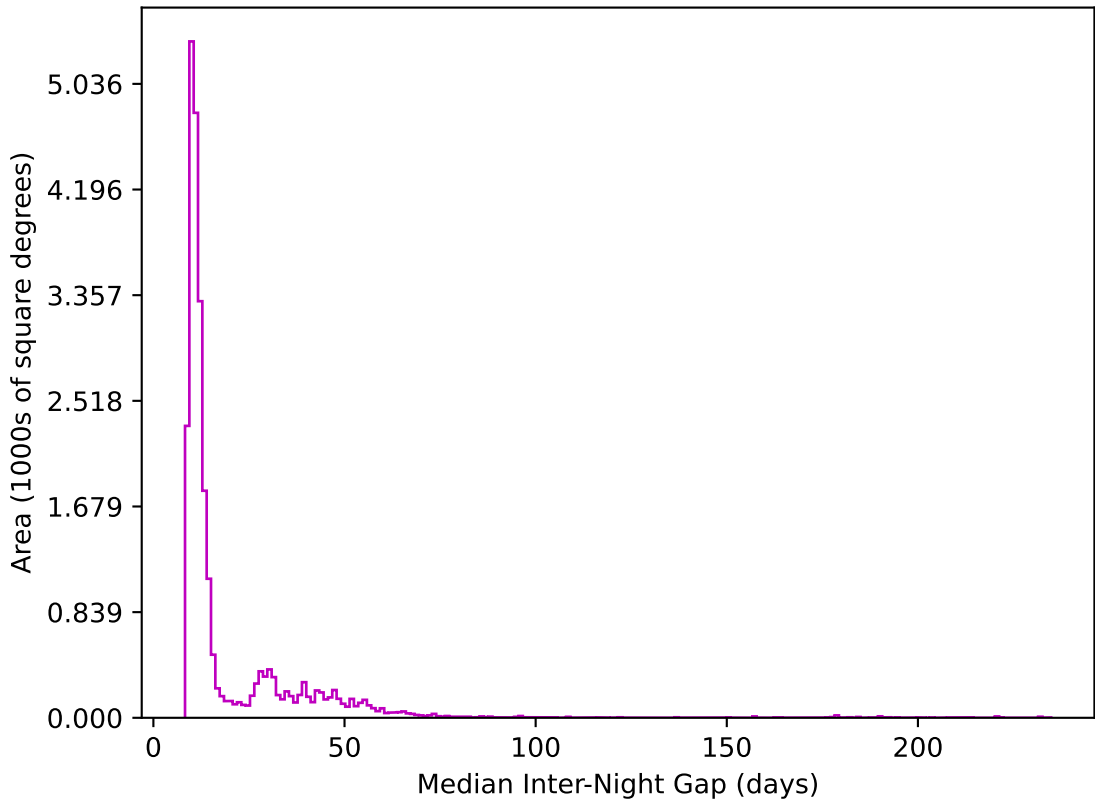
noroll_mjdp120_v3.4_10yrs All sky z band: Median Inter-Night Gap
