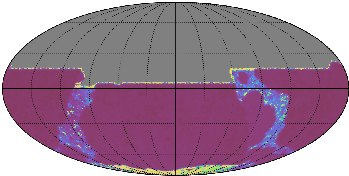
noroll_mjdp120_v3.4_10yrs All sky y band: Median Inter-Night Gap
