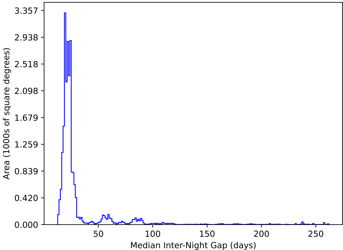
noroll_mjdp120_v3.4_10yrs All sky y band: Median Inter-Night Gap
