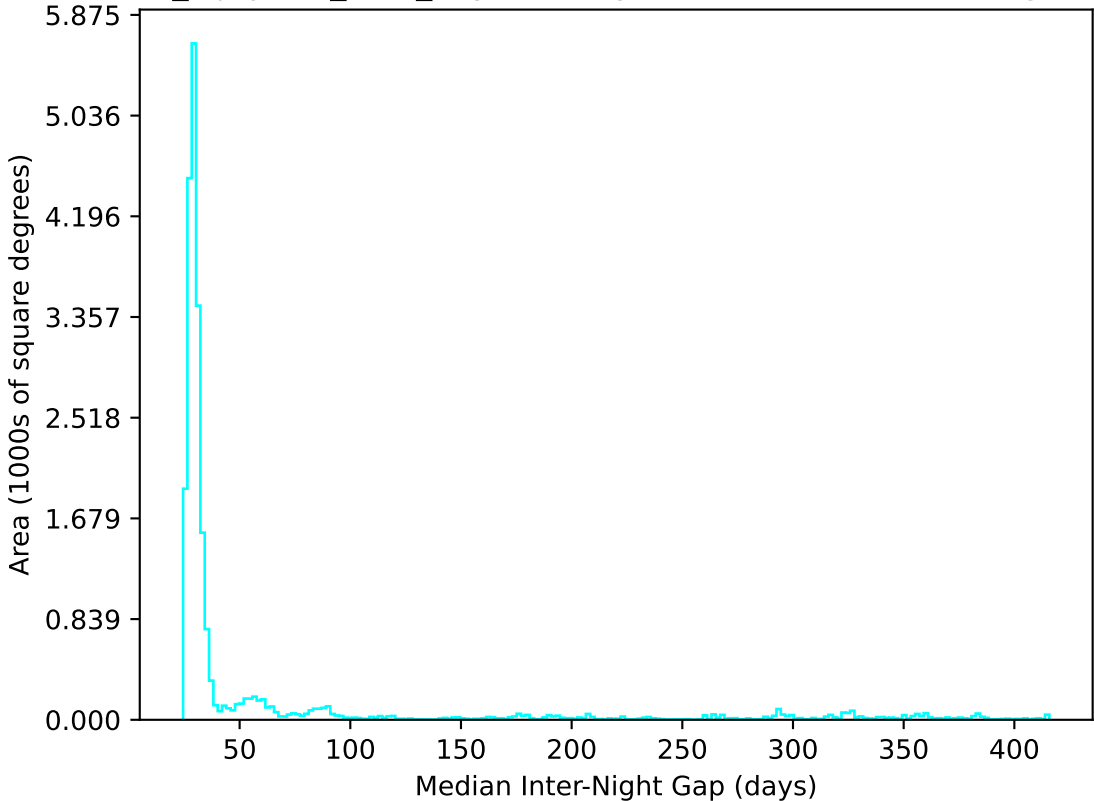
noroll_mjdp120_v3.4_10yrs All sky u band: Median Inter-Night Gap
