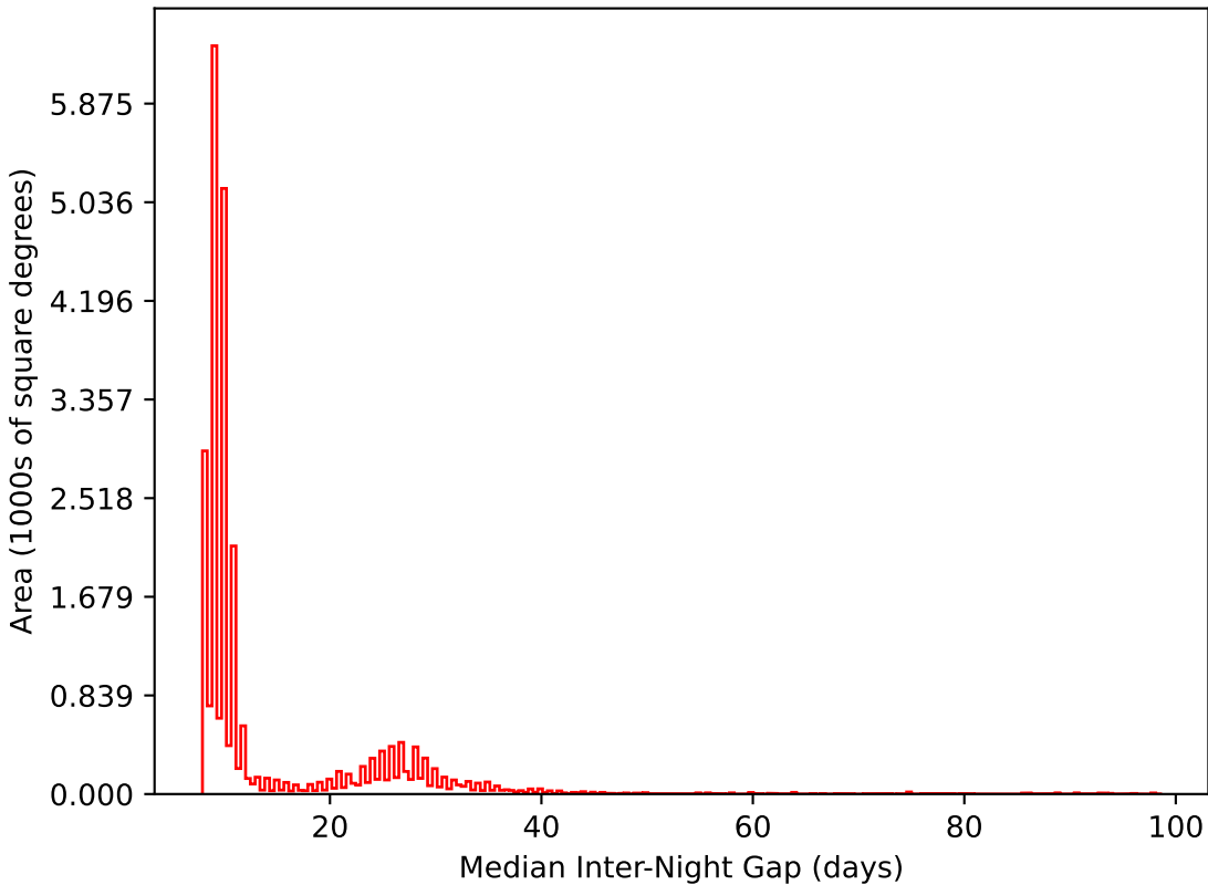
noroll_mjdp120_v3.4_10yrs All sky i band: Median Inter-Night Gap
