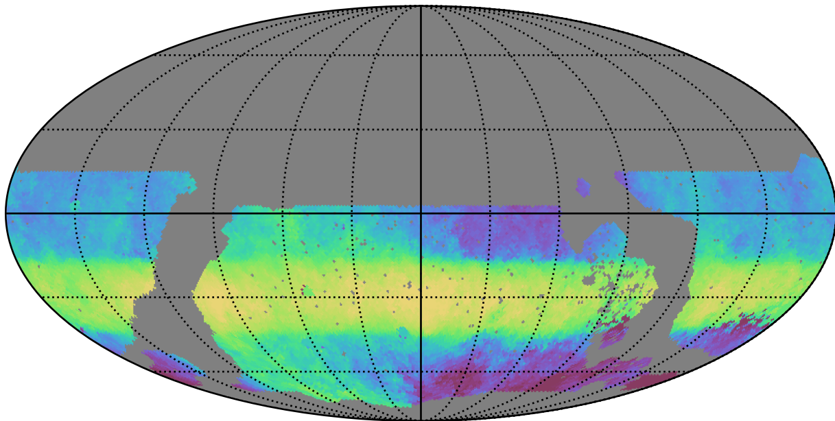
noroll_mjdp120_v3.4_10yrs WFD z band: Median HA
