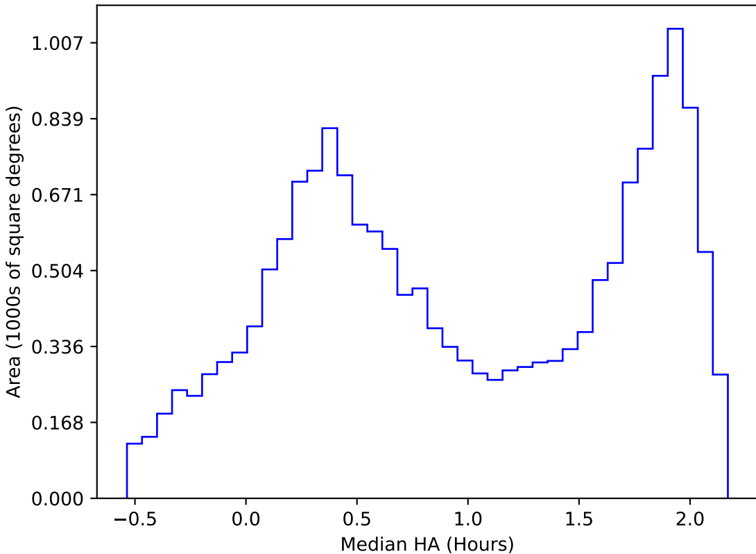
noroll_mjdp120_v3.4_10yrs WFD y band: Median HA
