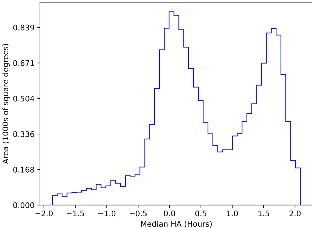
noroll_mjdp120_v3.4_10yrs WFD u band: Median HA
