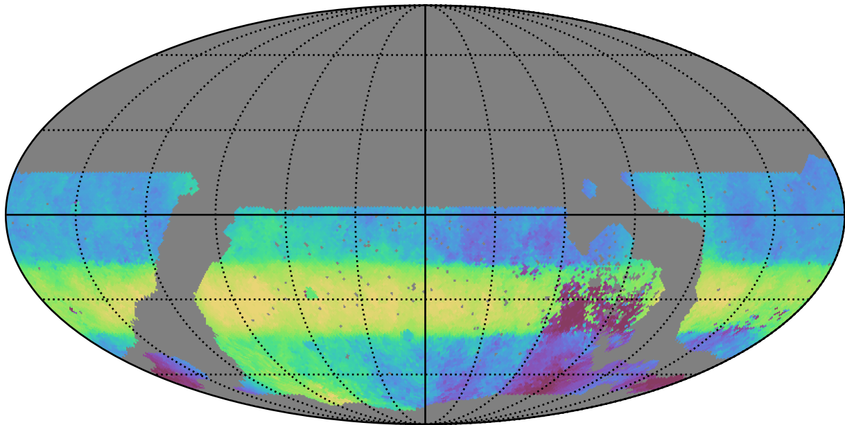
noroll_mjdp120_v3.4_10yrs WFD r band: Median HA
