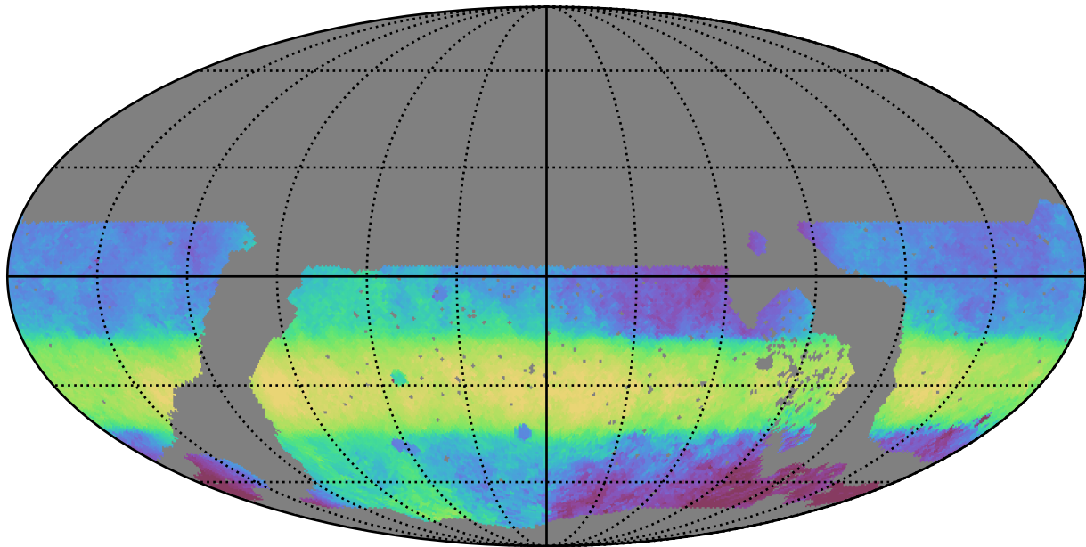
noroll_mjdp120_v3.4_10yrs WFD i band: Median HA
