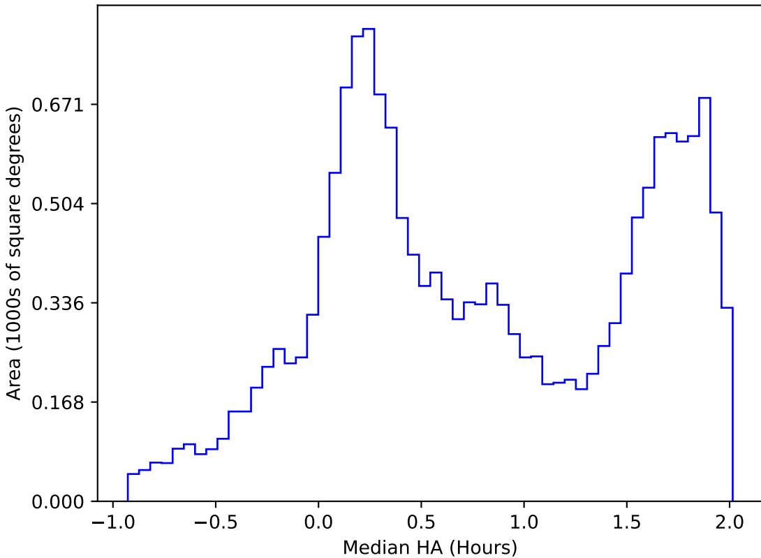
noroll_mjdp120_v3.4_10yrs WFD i band: Median HA
