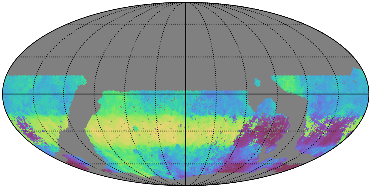
noroll_mjdp120_v3.4_10yrs WFD g band: Median HA
