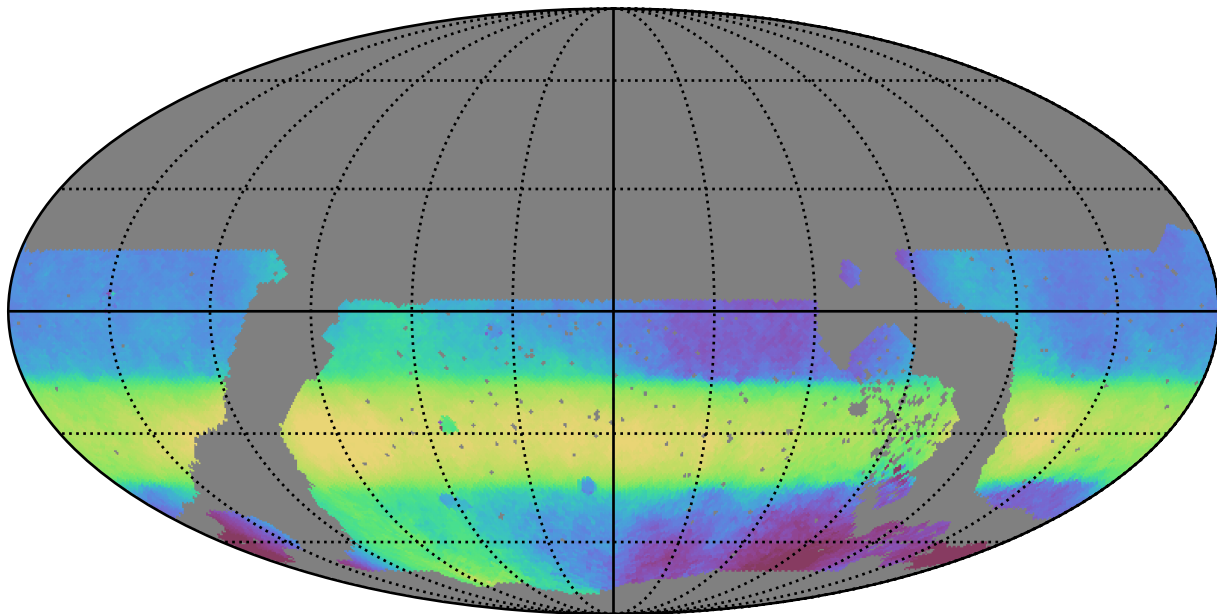
noroll_mjdp120_v3.4_10yrs WFD all bands: Median HA
