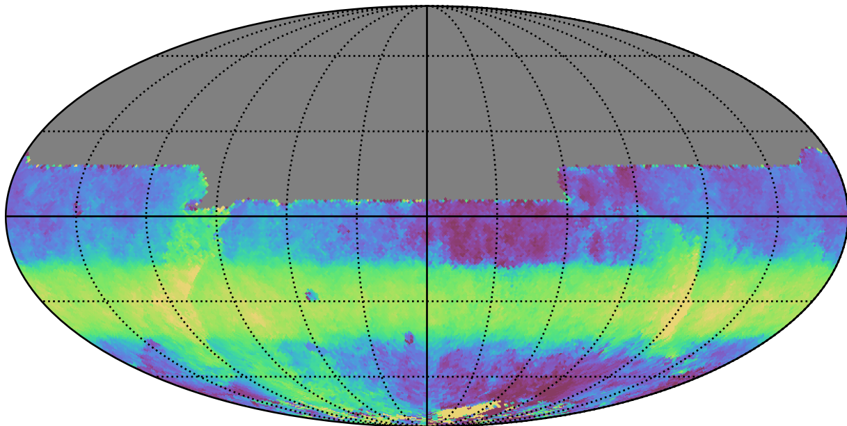
noroll_mjdp120_v3.4_10yrs All sky y band: Median HA
