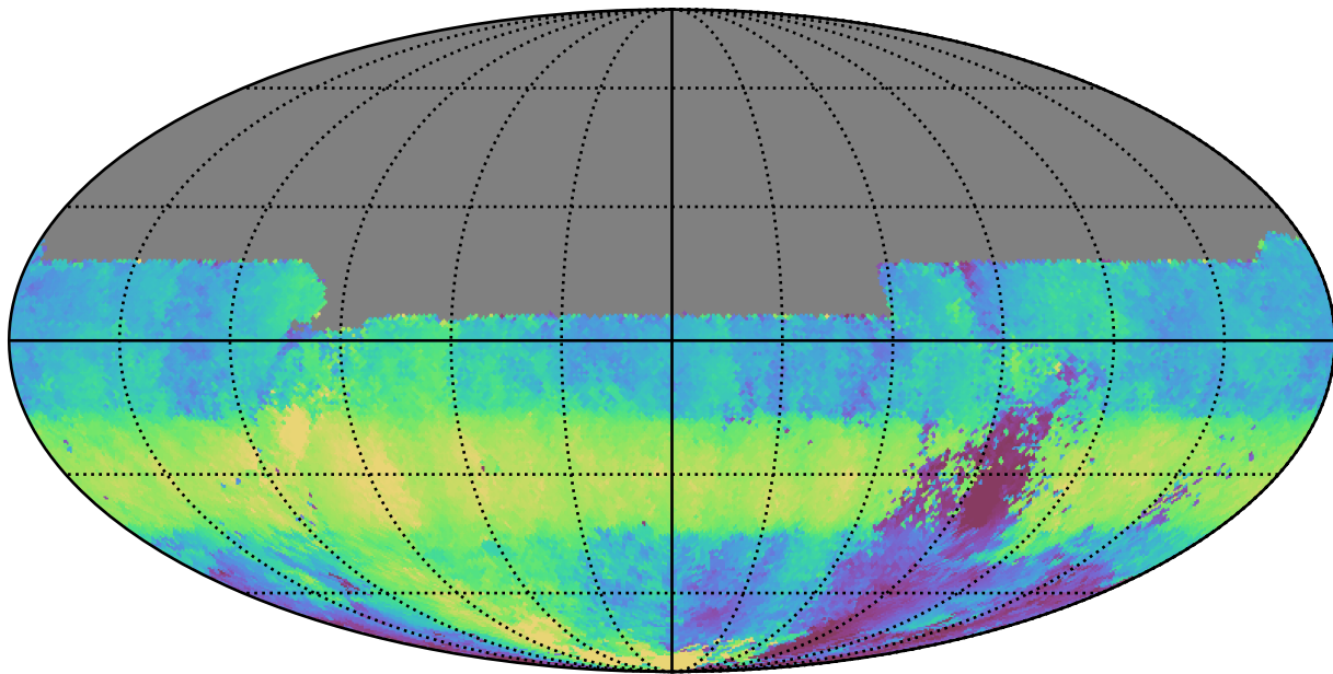
noroll_mjdp120_v3.4_10yrs All sky u band: Median HA
