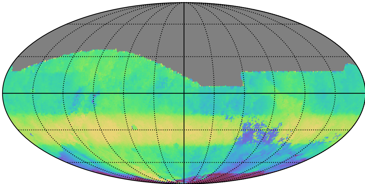
noroll_mjdp120_v3.4_10yrs All sky r band: Median HA
