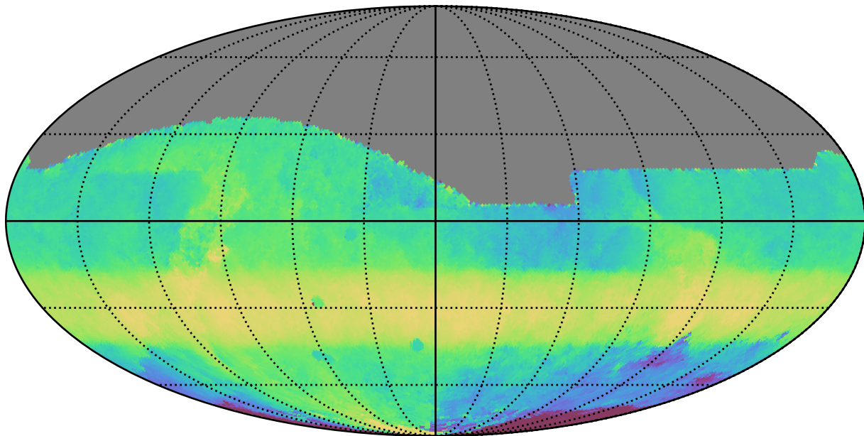
noroll_mjdp120_v3.4_10yrs All sky i band: Median HA
