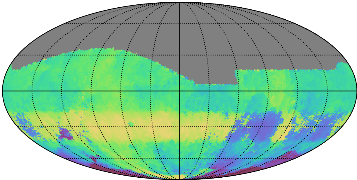
noroll_mjdp120_v3.4_10yrs All sky g band: Median HA
