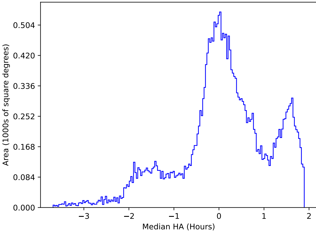
noroll_mjdp120_v3.4_10yrs All sky g band: Median HA
