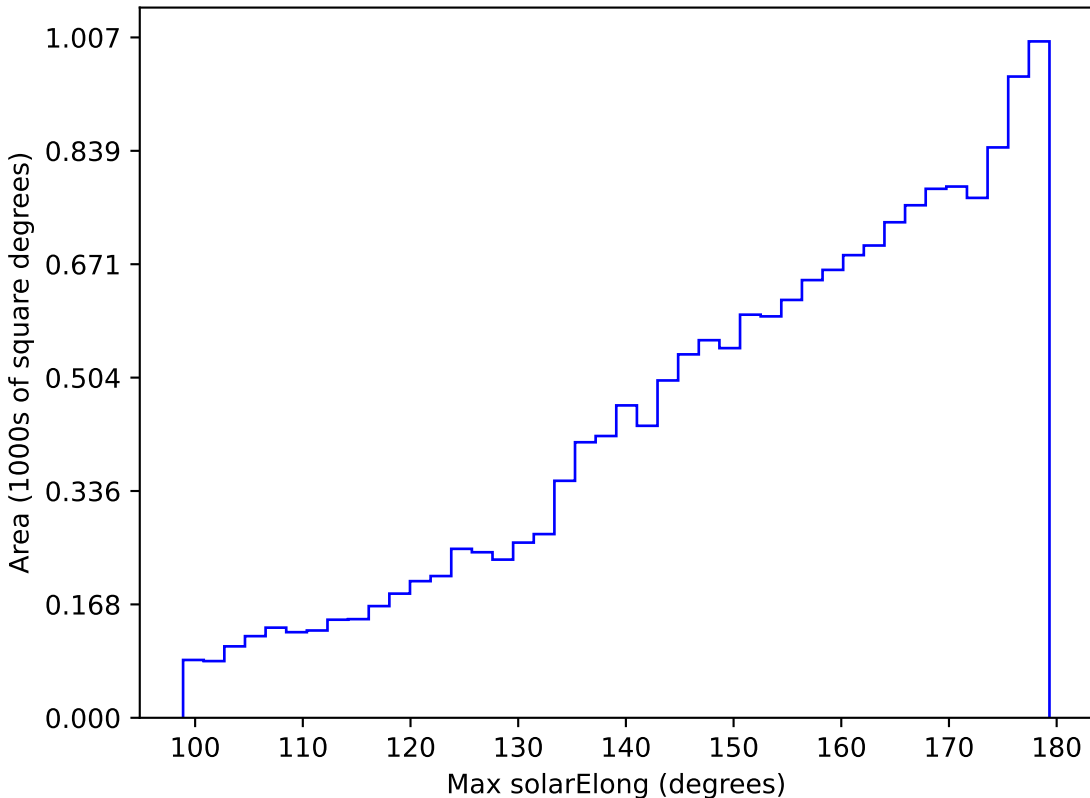
noroll_mjdp120_v3.4_10yrs WFD z band: Max solarElong
