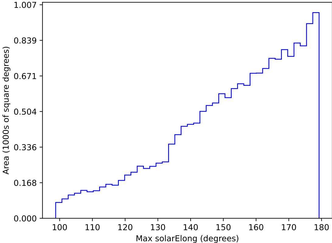
noroll_mjdp120_v3.4_10yrs WFD y band: Max solarElong
