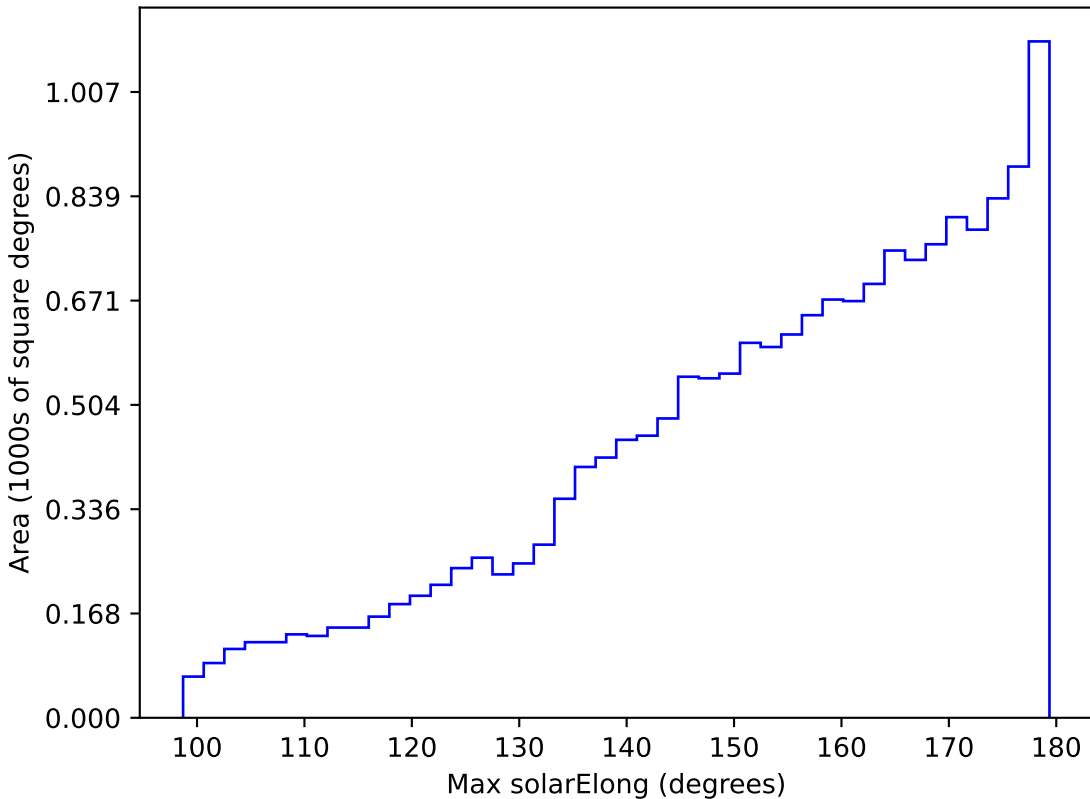
noroll_mjdp120_v3.4_10yrs WFD i band: Max solarElong
