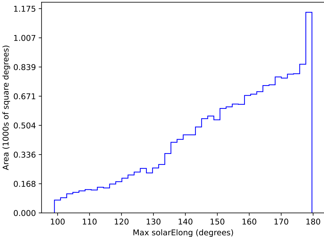
noroll_mjdp120_v3.4_10yrs WFD all bands: Max solarElong
