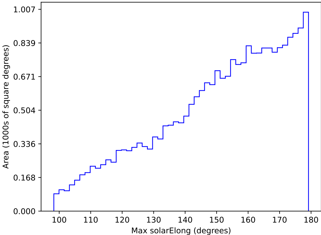
noroll_mjdp120_v3.4_10yrs All sky y band: Max solarElong
